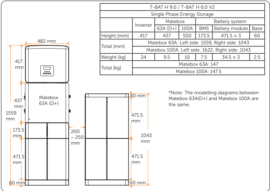
Three phase energy storage configuration examples (Dimension Unit: mm) X3-Hybrid G4 + X3 Matebox Basic + T-BAT-SYS-HV-3.0 / T-BAT-SYS-HV-3.0 V2
